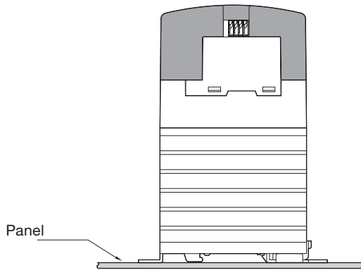
Horizontal Installation
