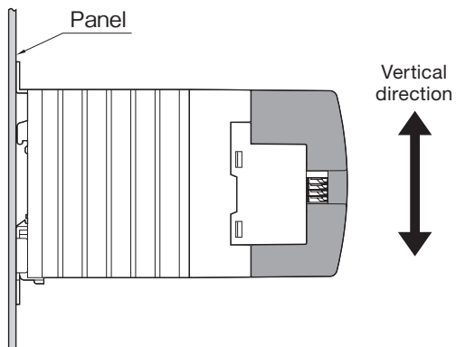
Vertical Installation
